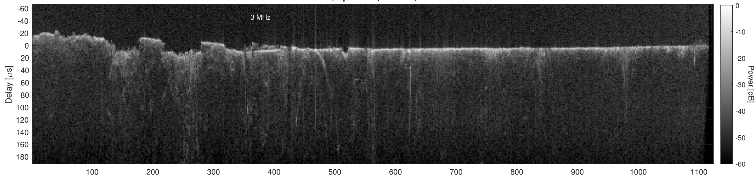
Orbit 12240, Cluttergram
