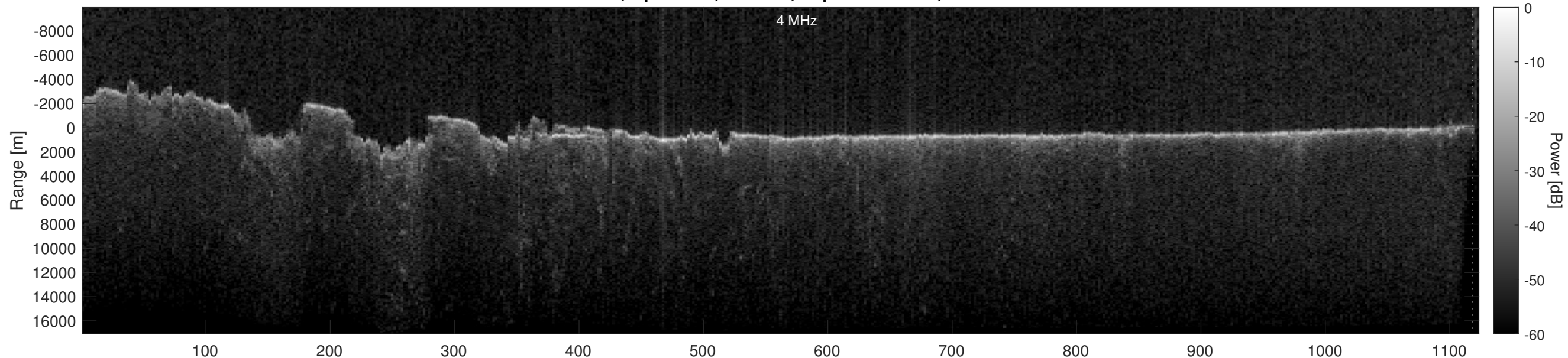
Orbit 12240, Optimized, Window, Depth-Corrected, Channel 2
