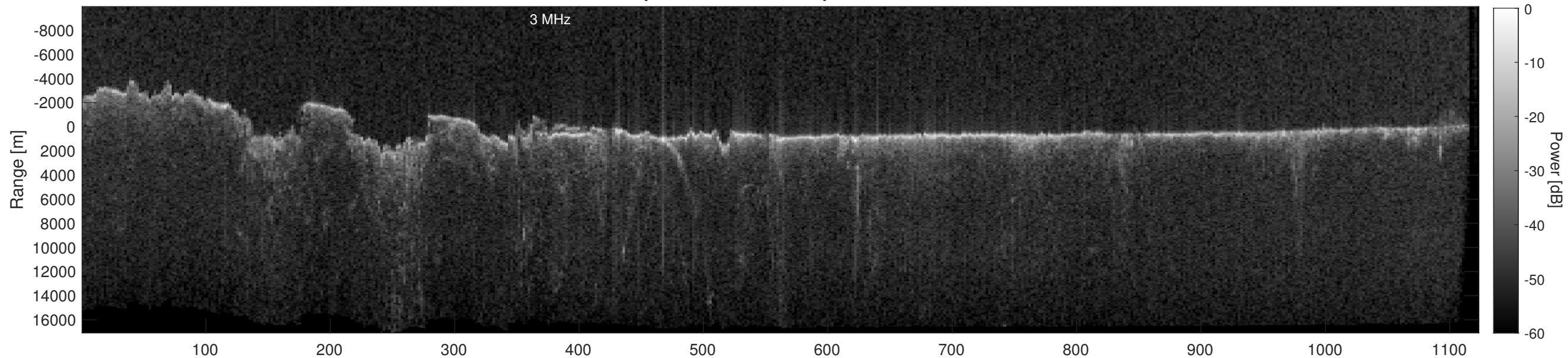
Orbit 12240, Depth-Corrected Cluttergram
