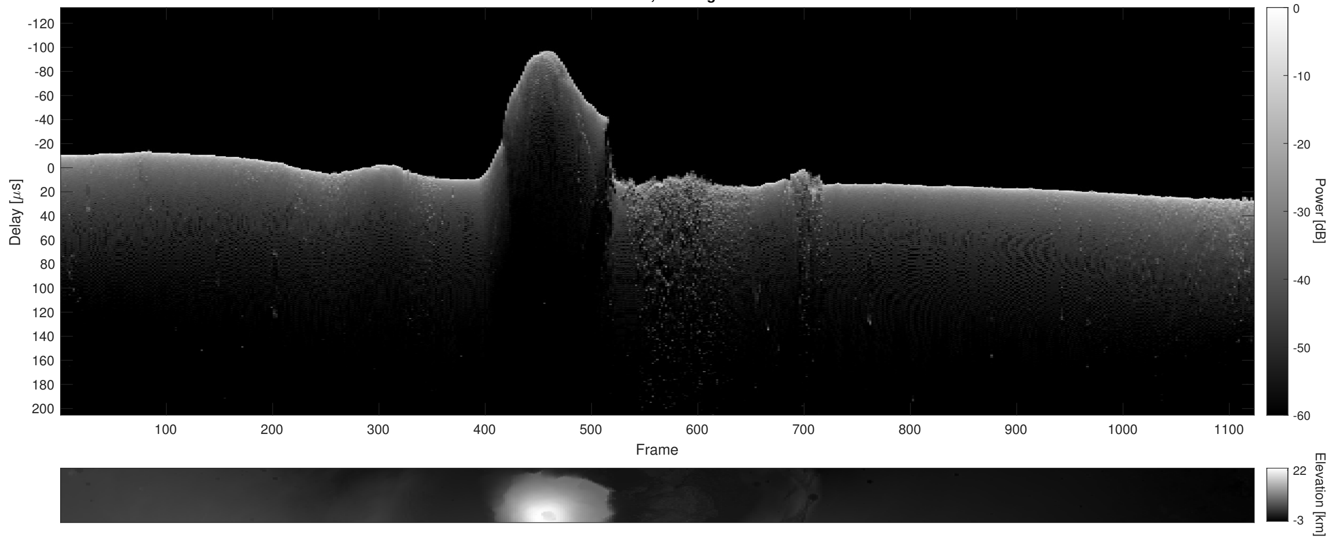
Orbit 12241, Cluttergram
