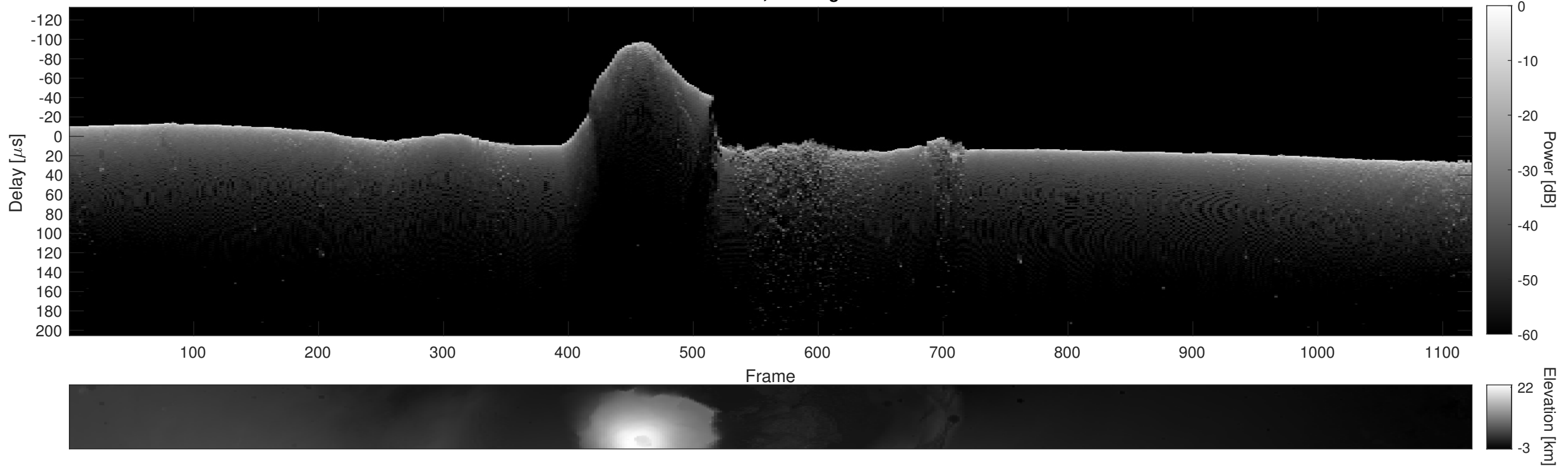
Orbit 12241, Cluttergram
