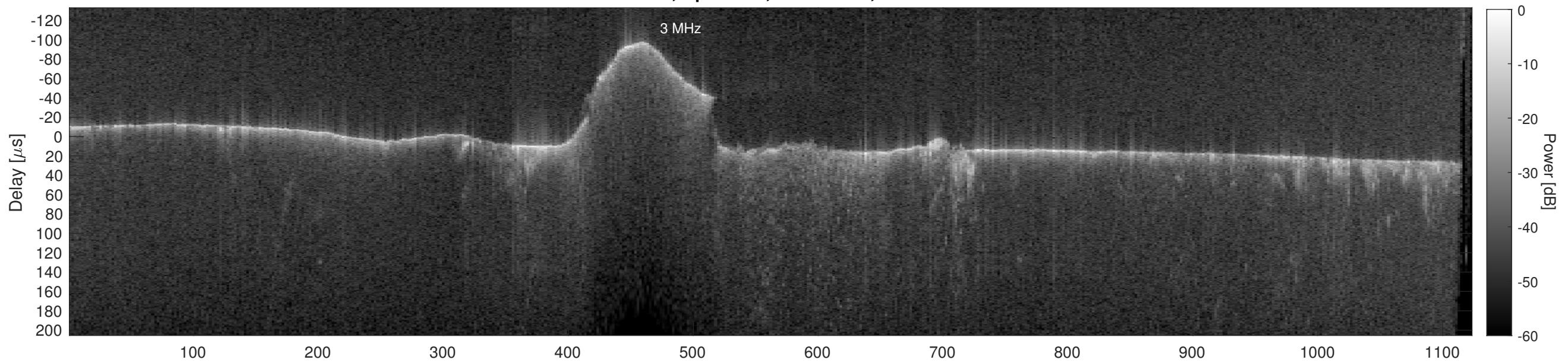
Orbit 12241, Cluttergram
