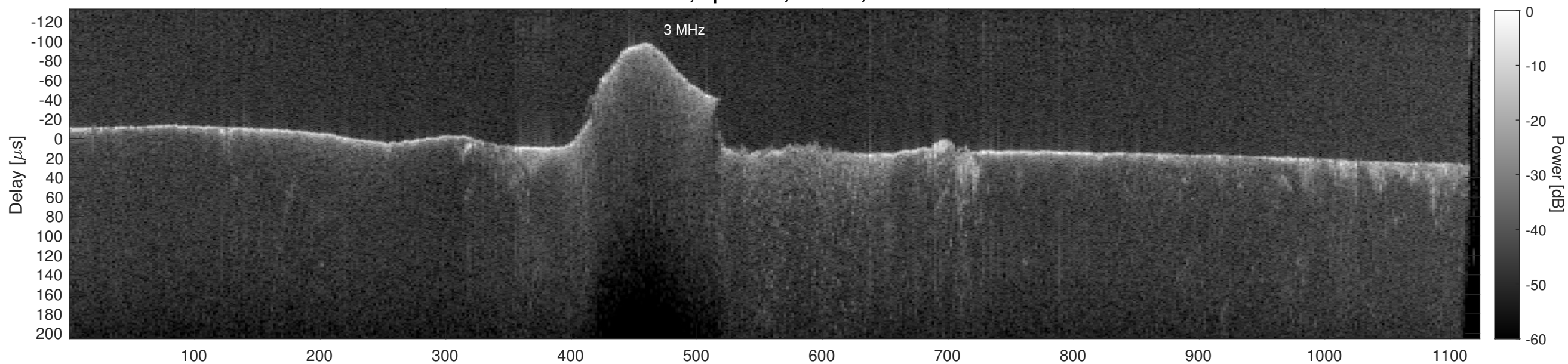
Orbit 12241, Cluttergram
