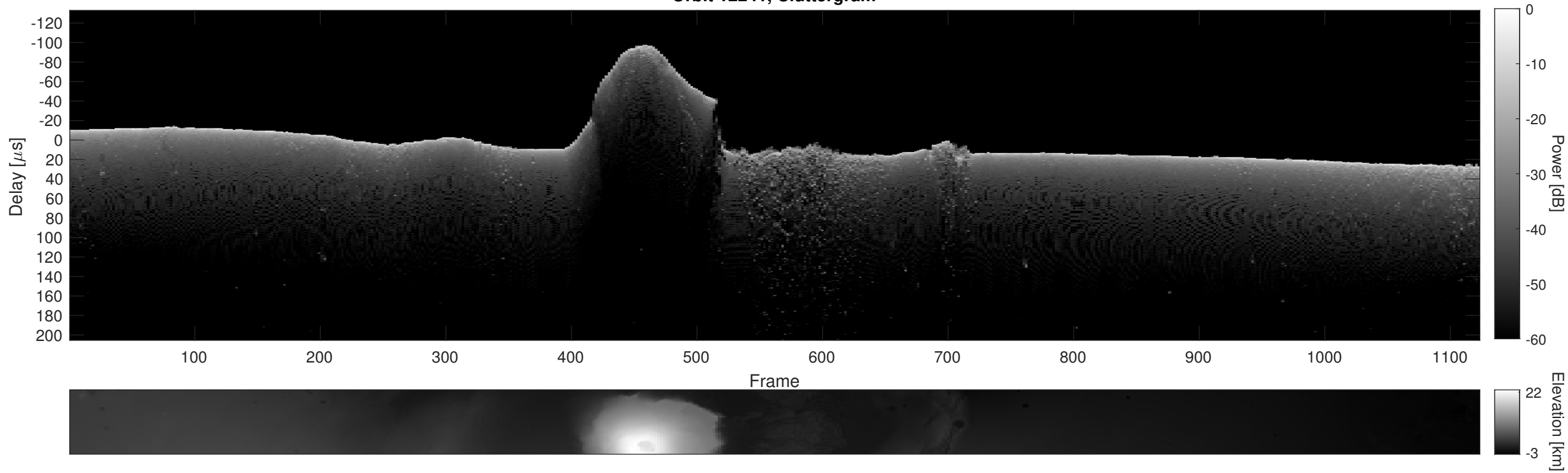
Orbit 12241, Cluttergram
