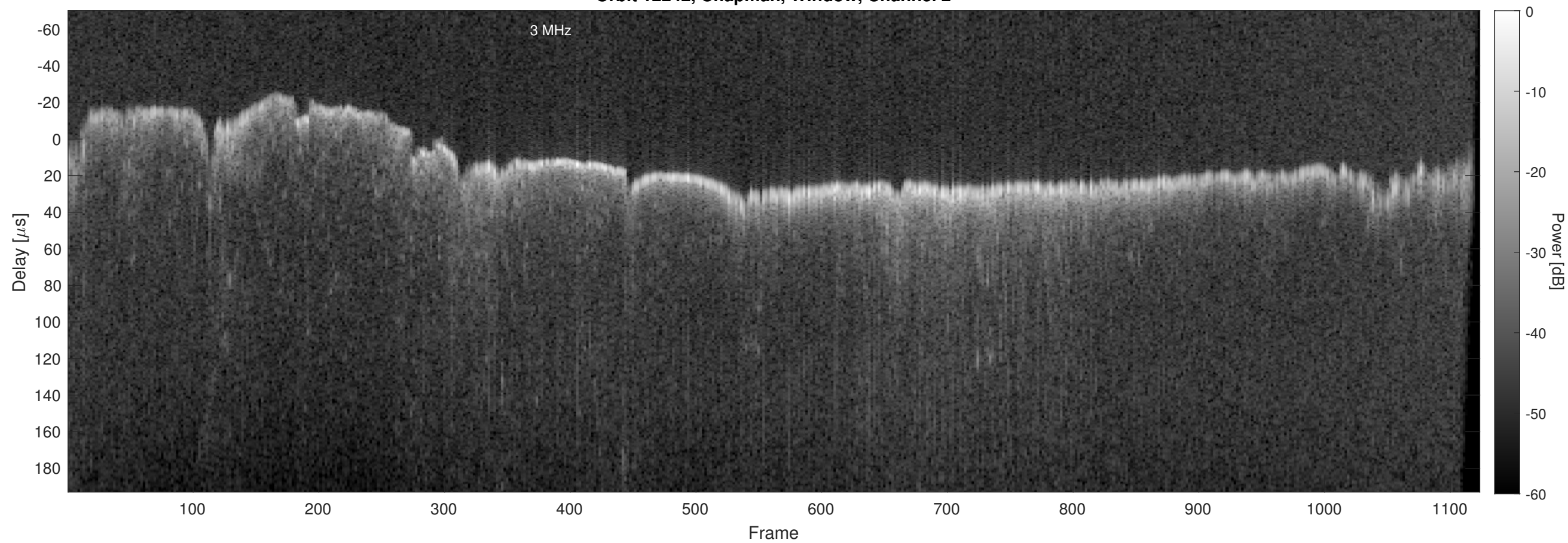
Orbit 12242, Chapman, Window, Channel 2
