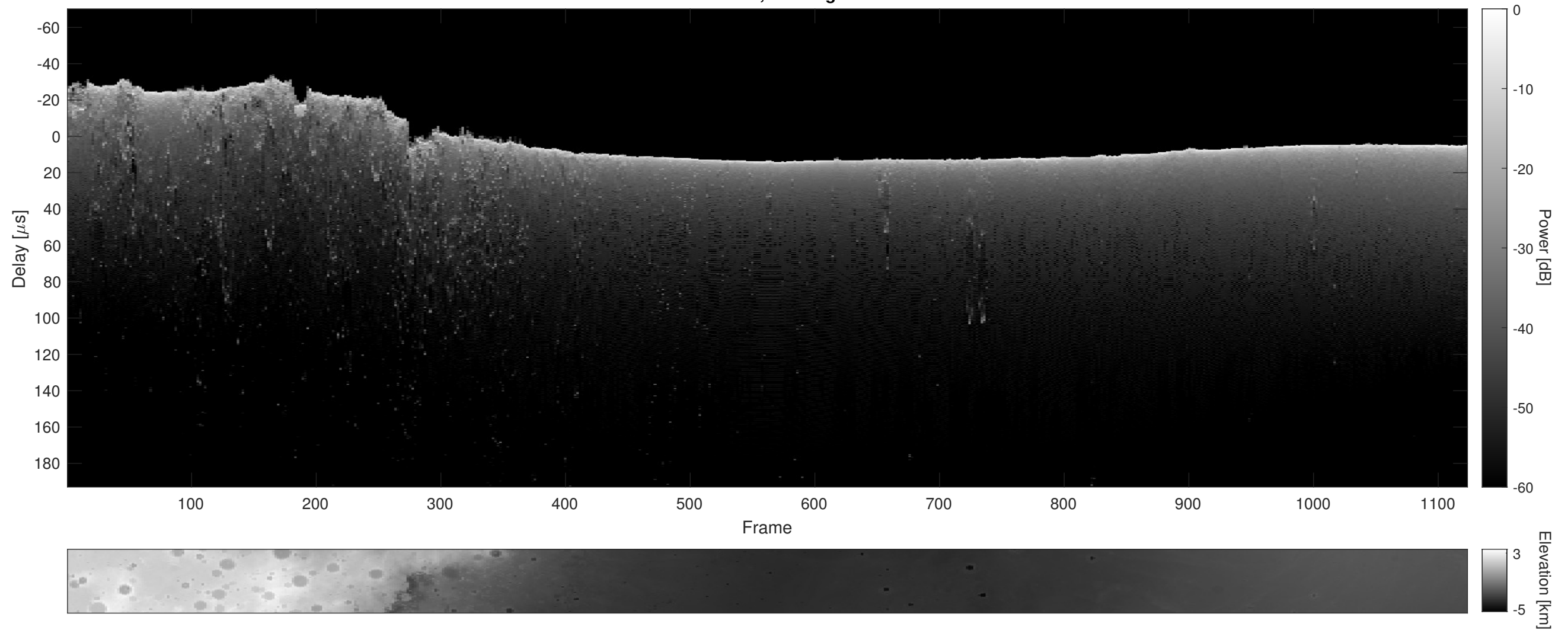
Orbit 12242, Cluttergram
