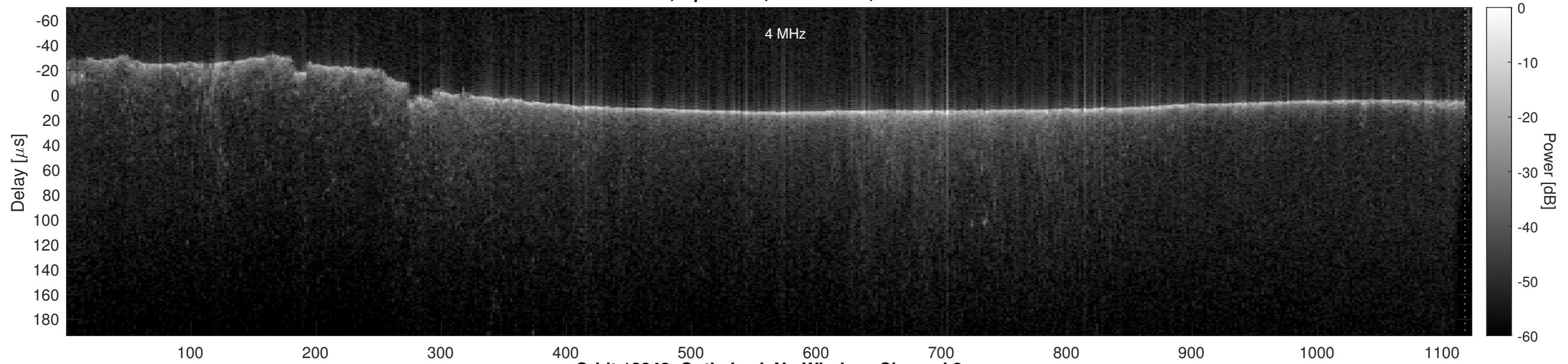
Orbit 12242, Optimized, No Window, Channel 2
