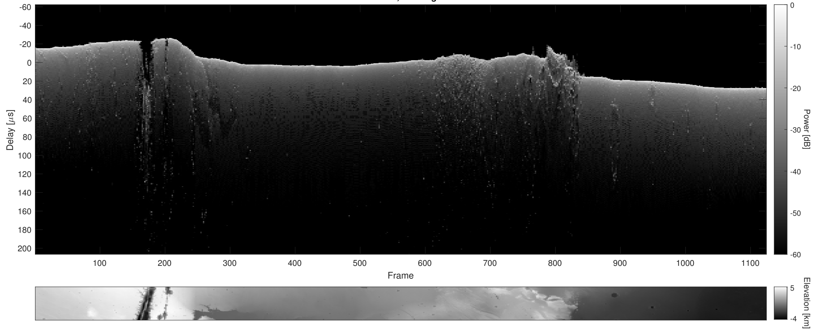
Orbit 12244, Cluttergram
