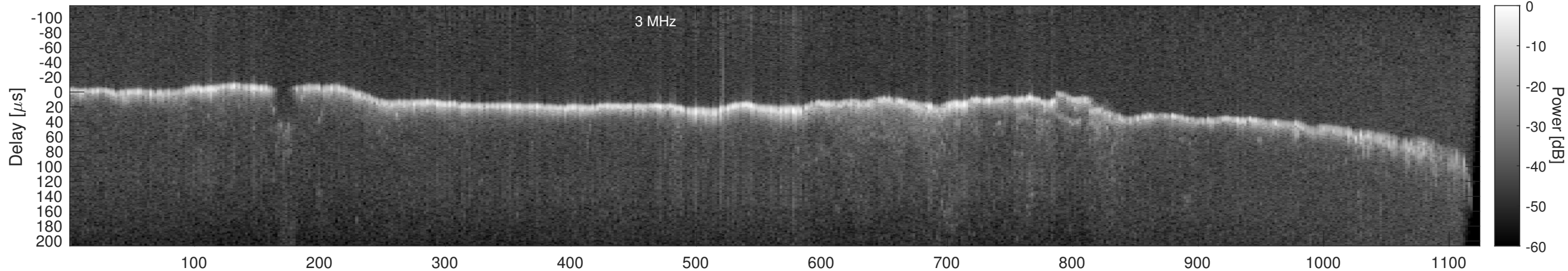
Orbit 12244, Window, Channel 2, Chapman
