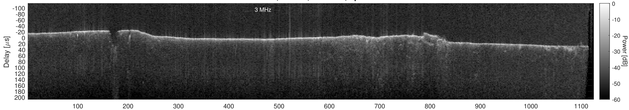
Orbit 12244, Cluttergram
