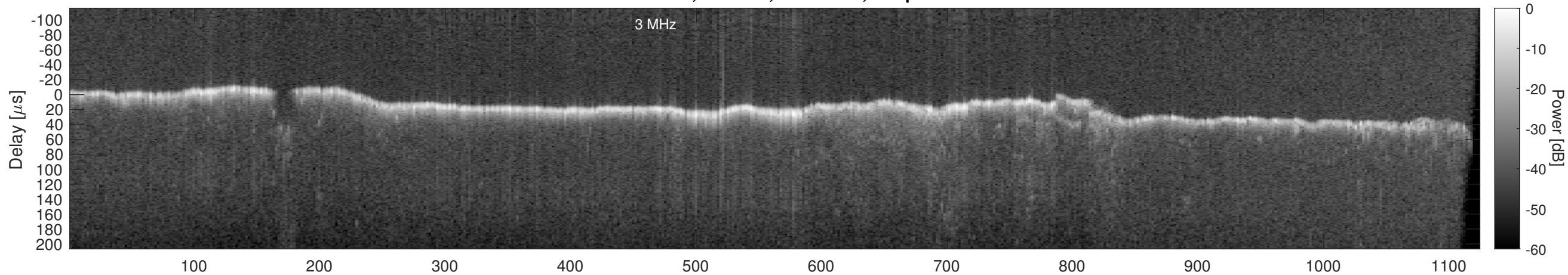
Orbit 12244, Window, Channel 2, Optimized
