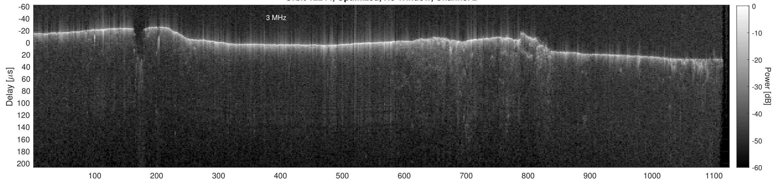
Orbit 12244, Cluttergram
