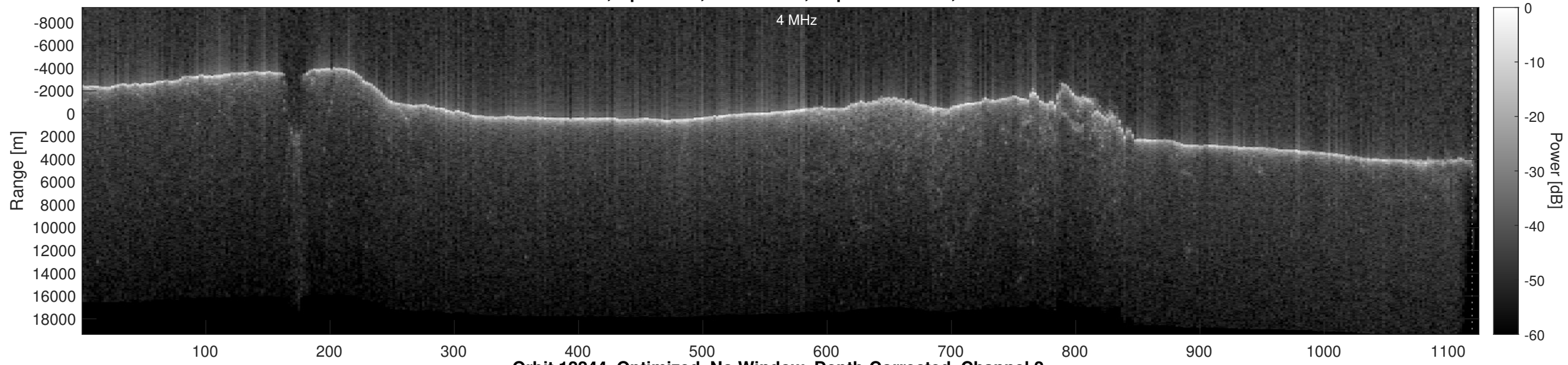
Orbit 12244, Optimized, No Window, Depth-Corrected, Channel 2
