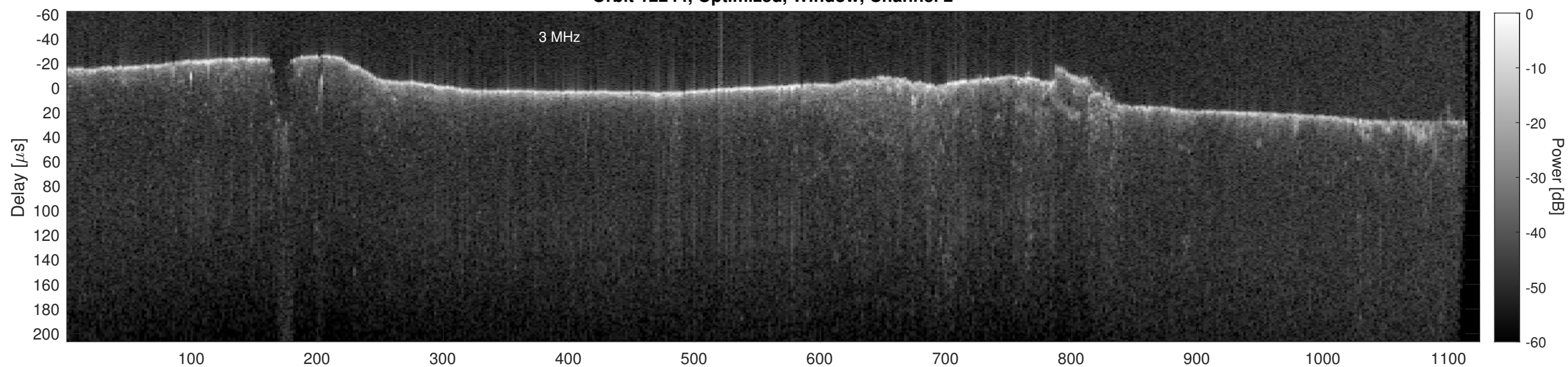
Orbit 12244, Cluttergram
