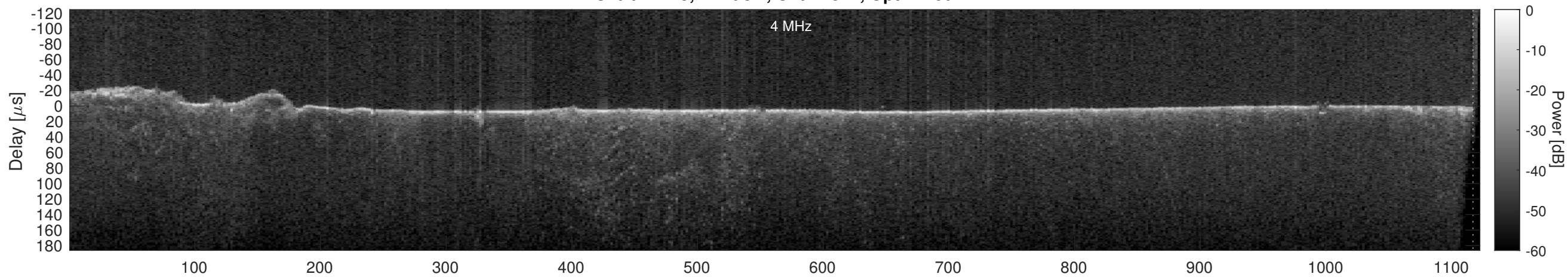
Orbit 12245, Cluttergram
