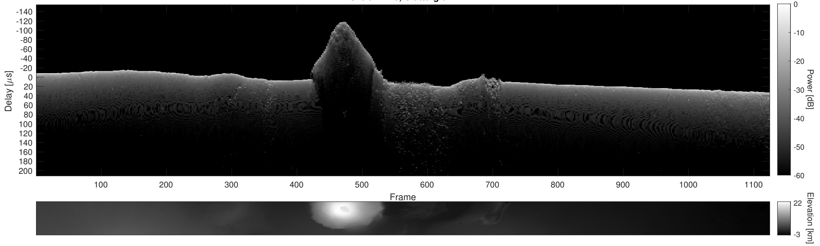
Orbit 12248, Cluttergram
