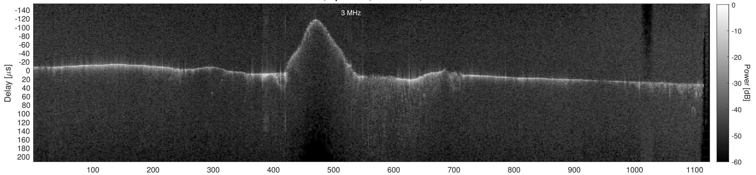
Orbit 12248, Cluttergram
