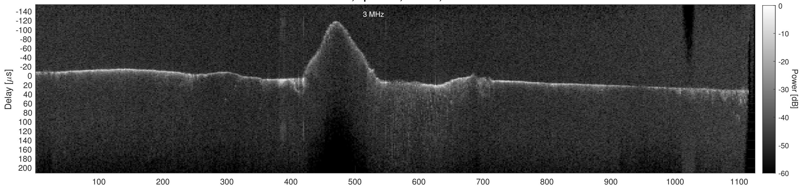
Orbit 12248, Cluttergram
