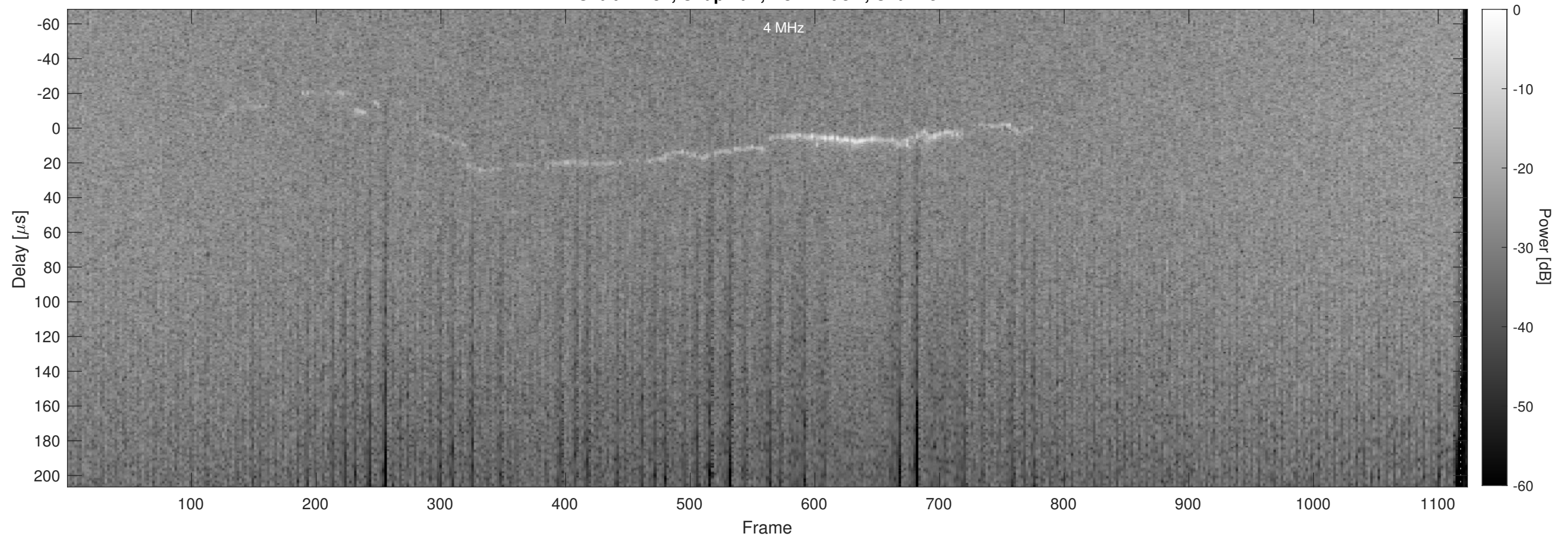
Orbit 12251, Chapman, No Window, Channel 2
