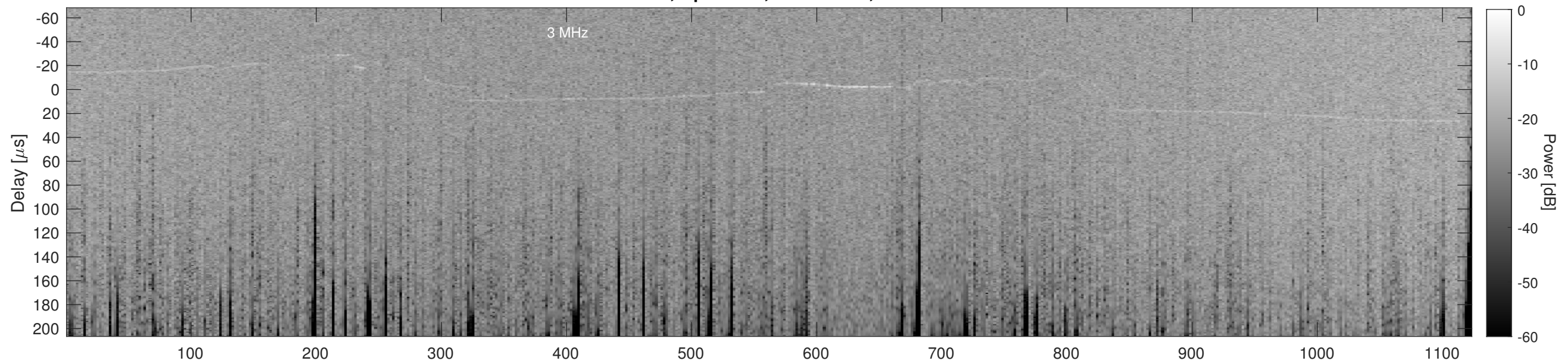
Orbit 12251, Cluttergram
