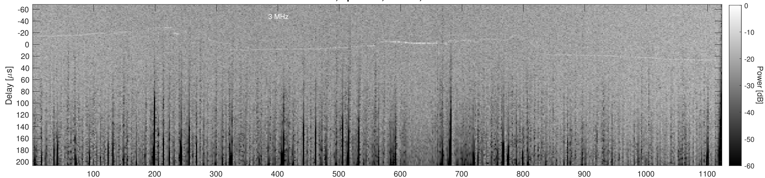
Orbit 12251, Cluttergram
