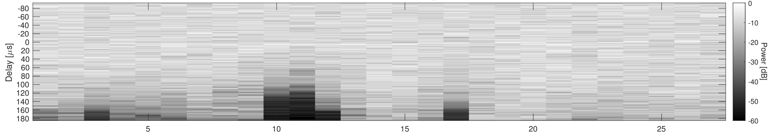
Orbit 12253, Cluttergram
