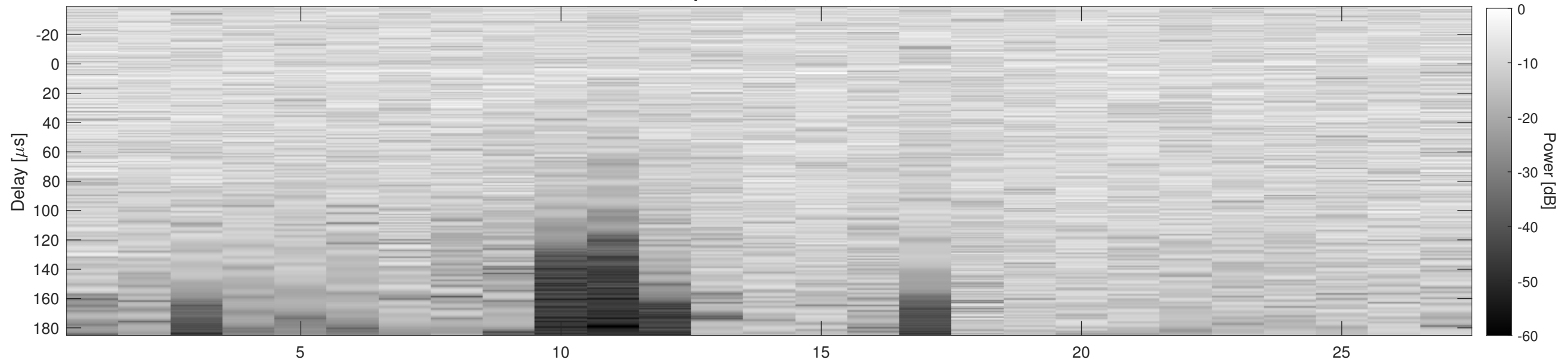
Orbit 12253, Cluttergram
