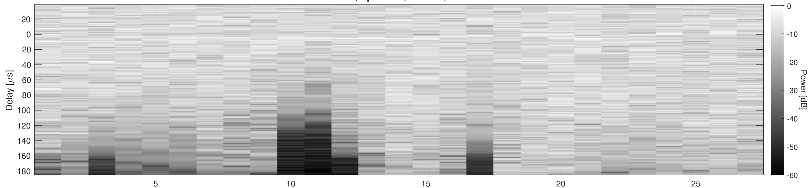
Orbit 12253, Cluttergram
