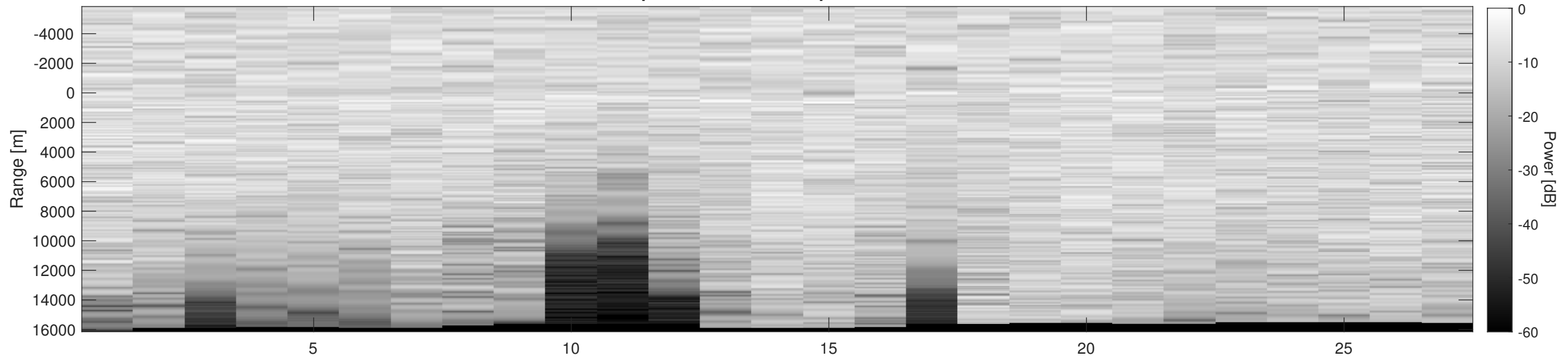
Orbit 12253, Depth-Corrected Cluttergram
