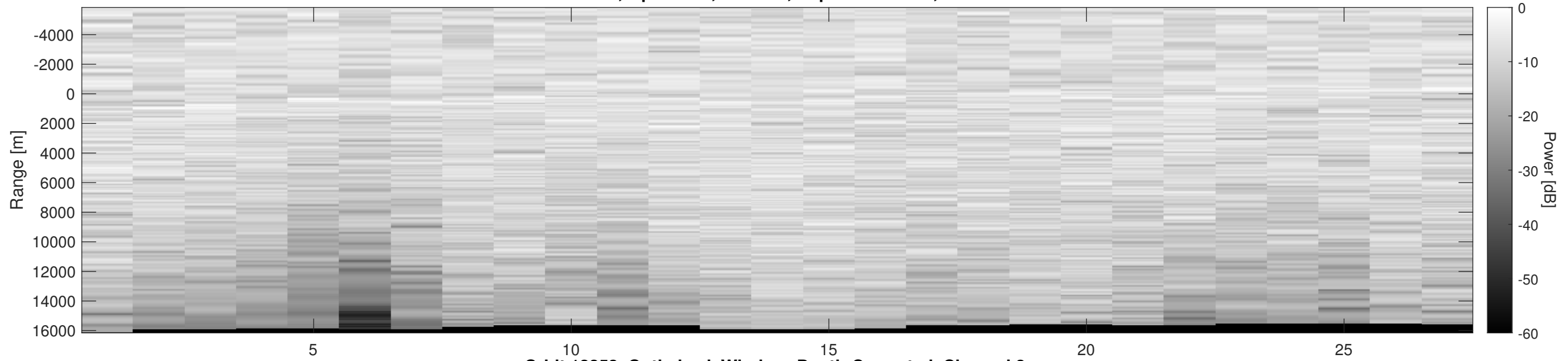
Orbit 12253, Optimized, Window, Depth-Corrected, Channel 2
