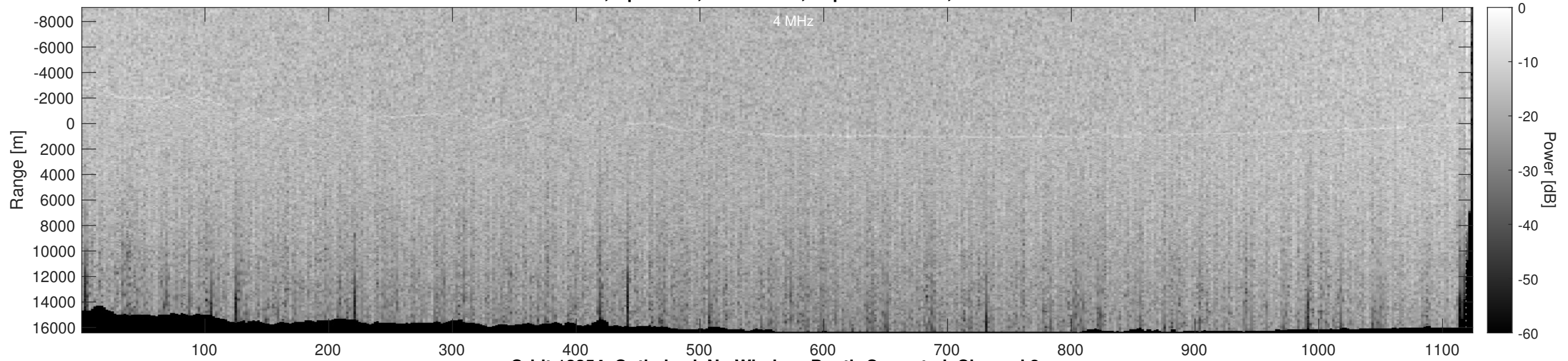
Orbit 12254, Optimized, No Window, Depth-Corrected, Channel 2
