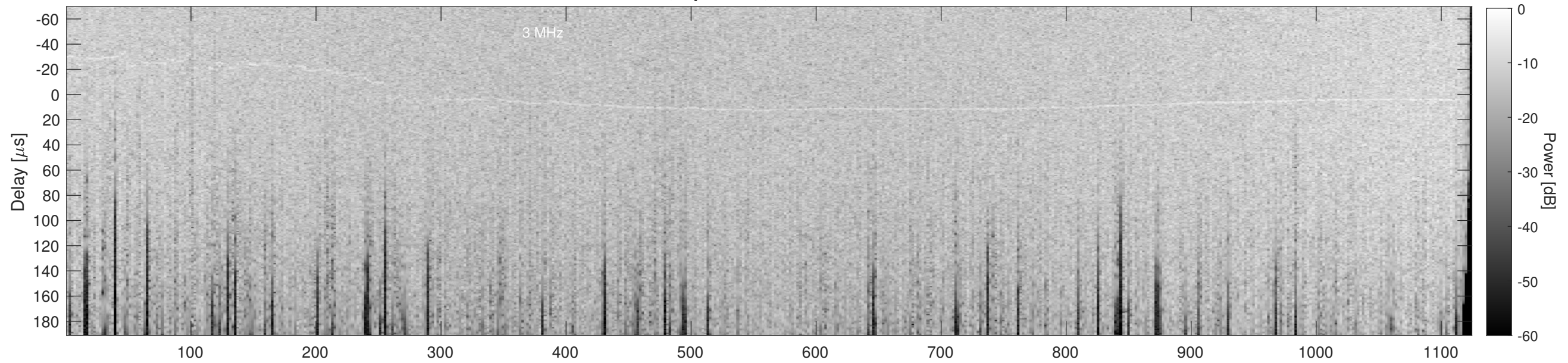
Orbit 12256, Cluttergram
