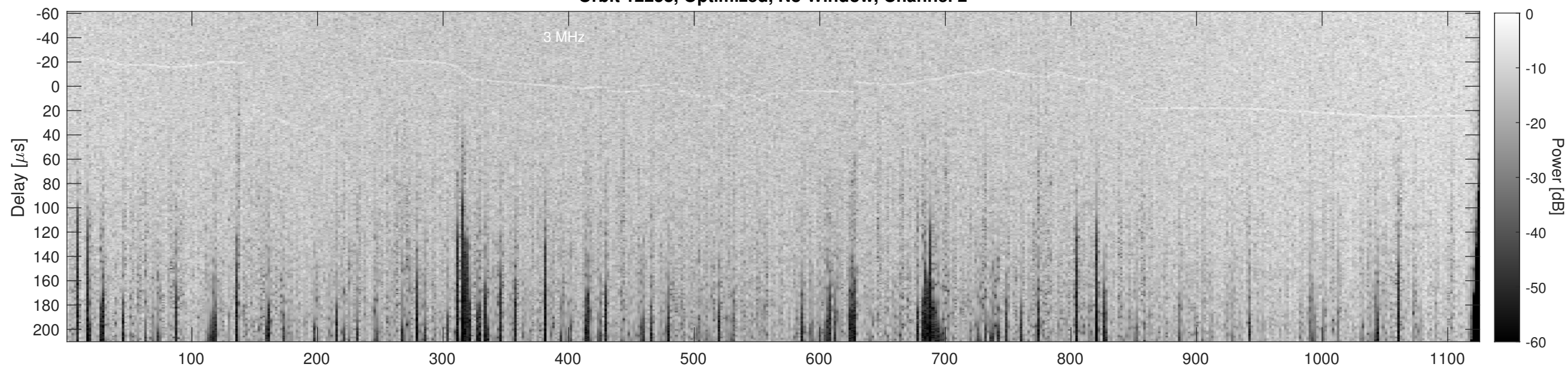
Orbit 12258, Cluttergram
