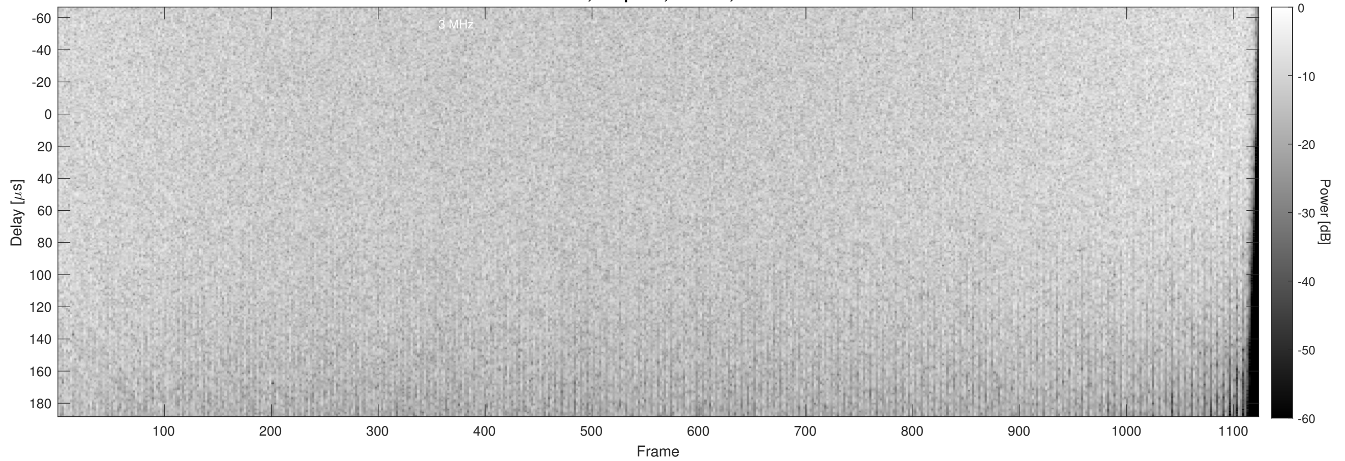
Orbit 12259, Chapman, Window, Channel 2
