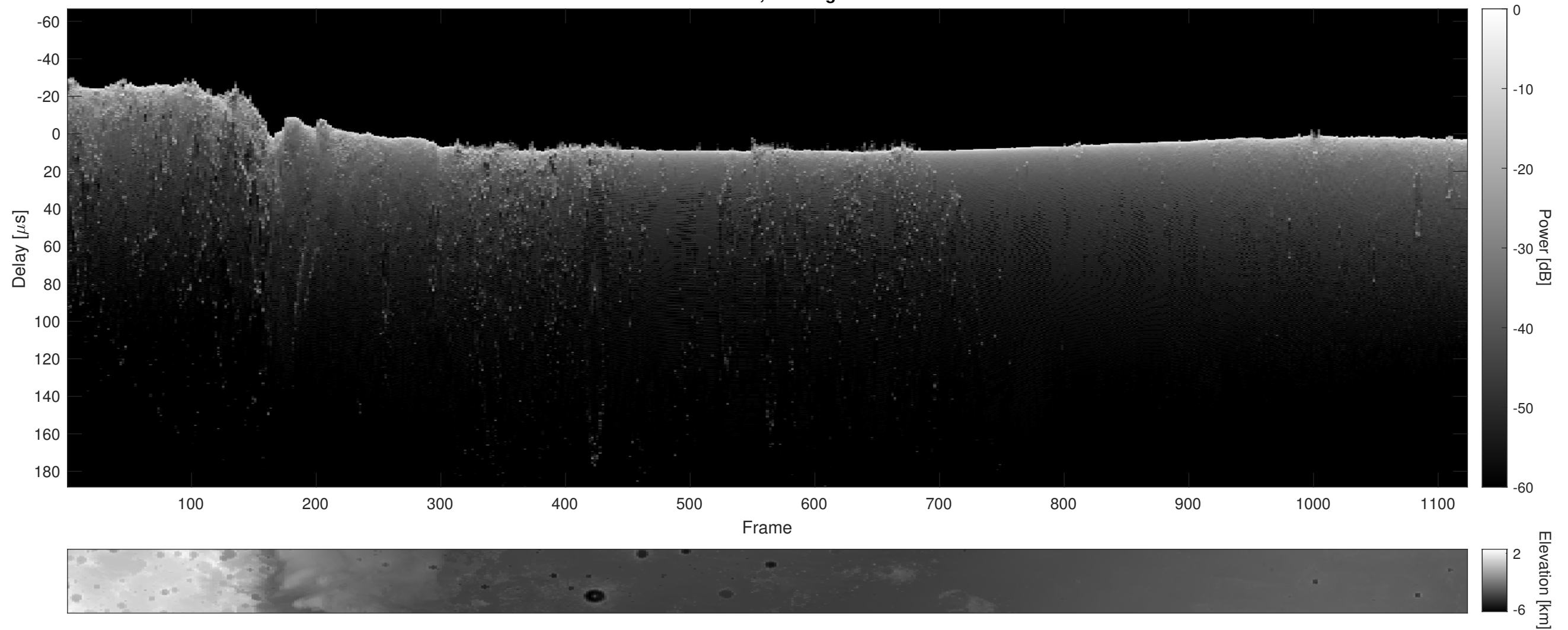
Orbit 12259, Cluttergram
