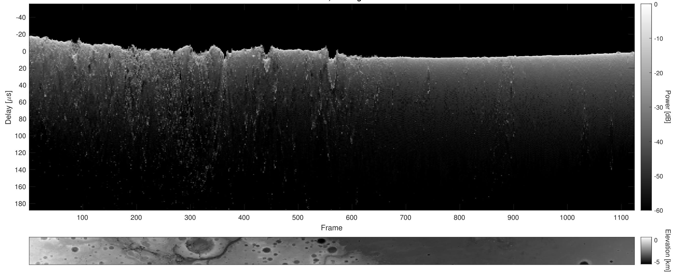
Orbit 12261, Cluttergram
