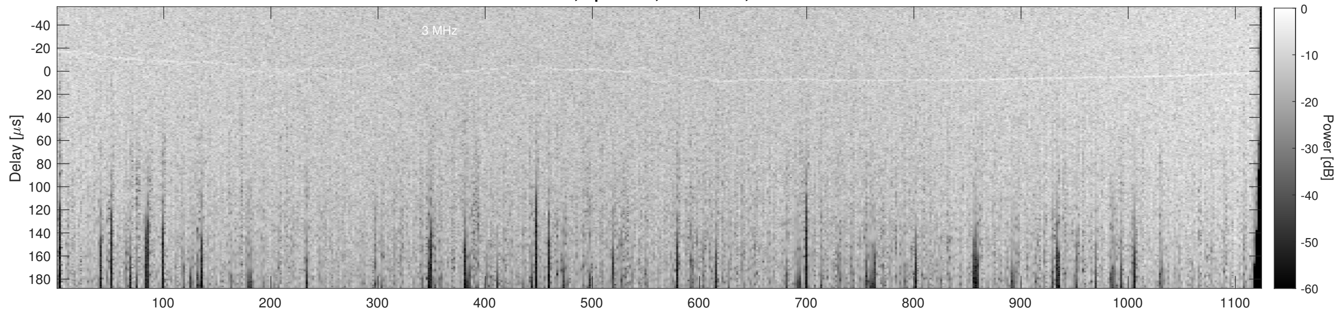
Orbit 12261, Cluttergram
