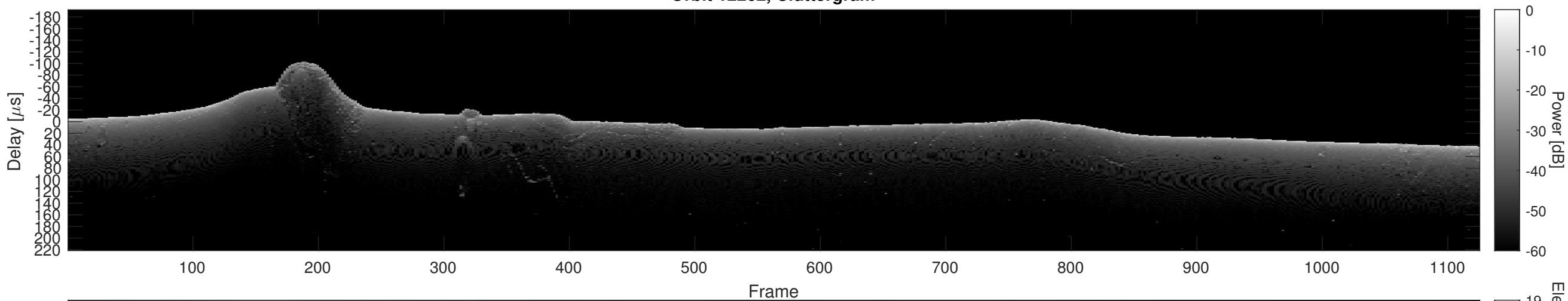
Orbit 12262, Cluttergram
