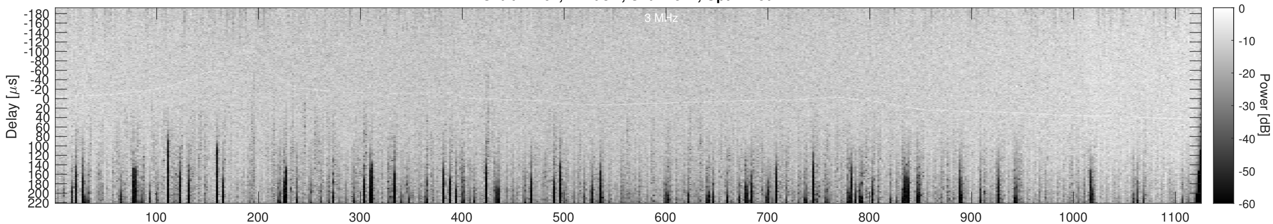
Orbit 12262, Cluttergram
