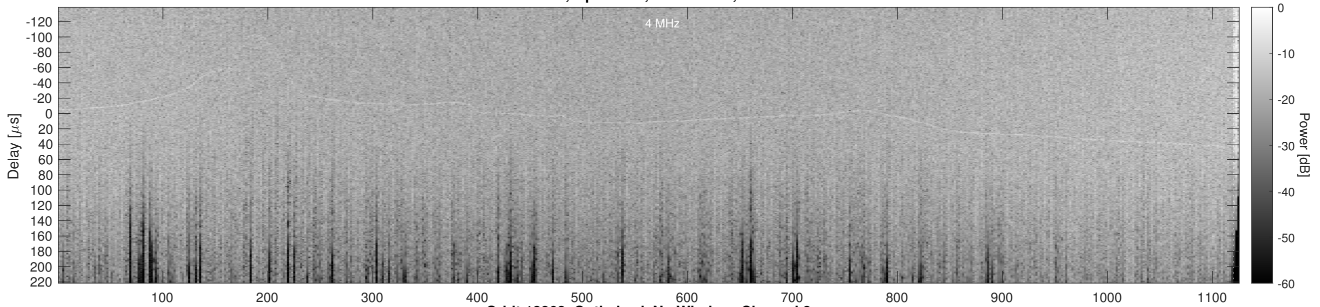
Orbit 12262, Optimized, No Window, Channel 2
