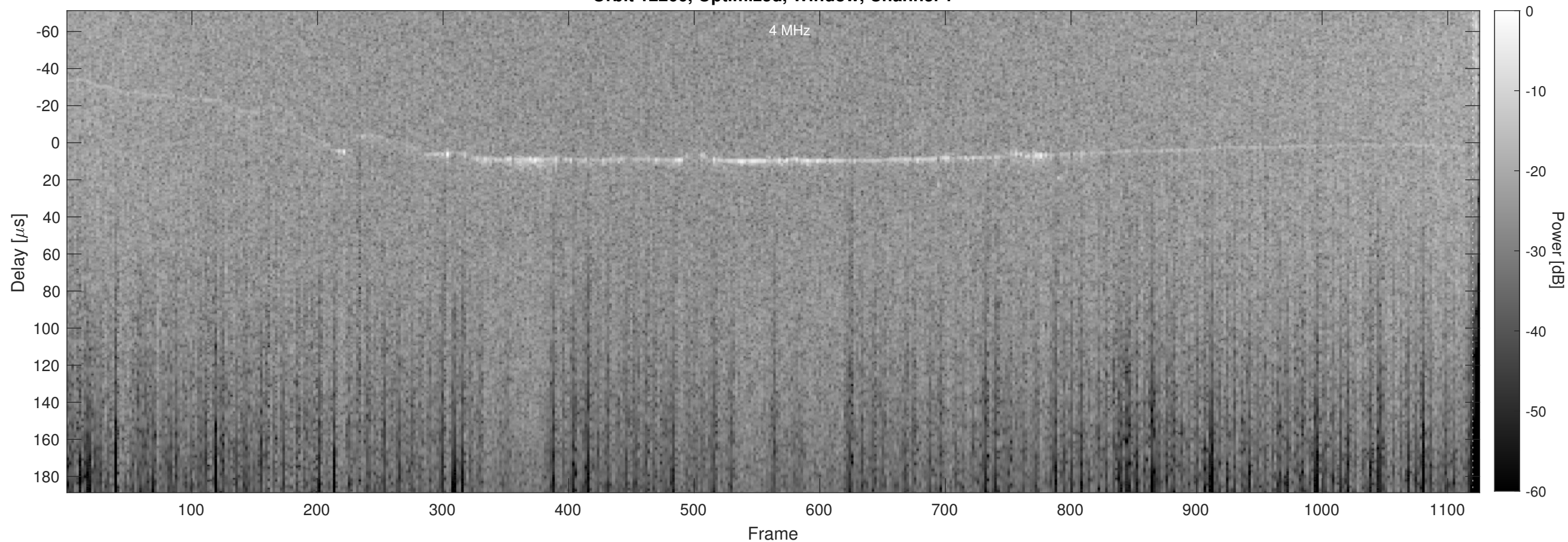
Orbit 12266, Optimized, Window, Channel 2
