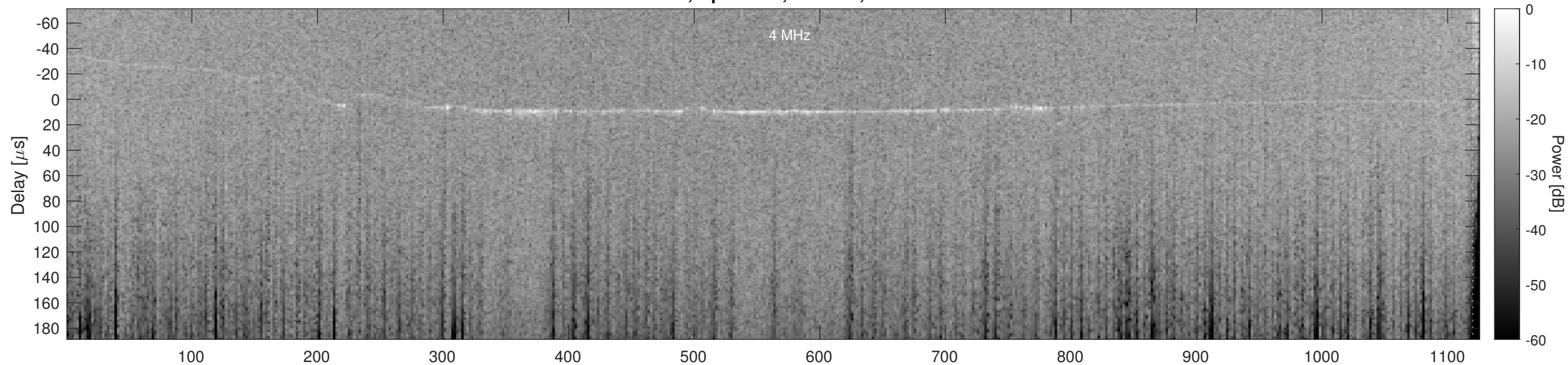
Orbit 12266, Optimized, Window, Channel 2
