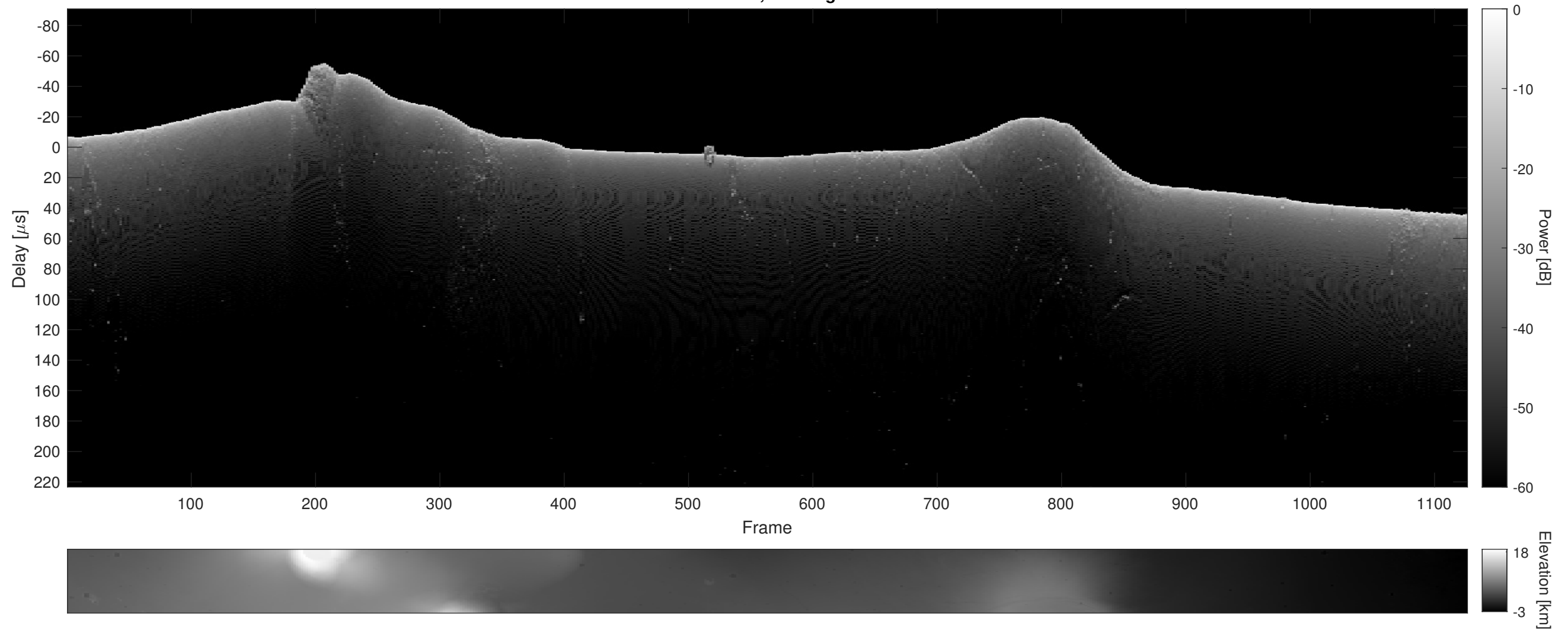
Orbit 12269, Cluttergram
