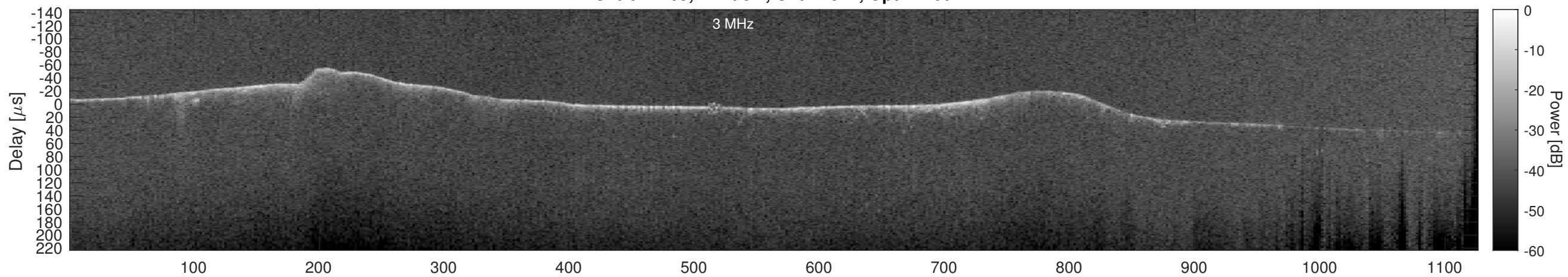
Orbit 12269, Cluttergram
