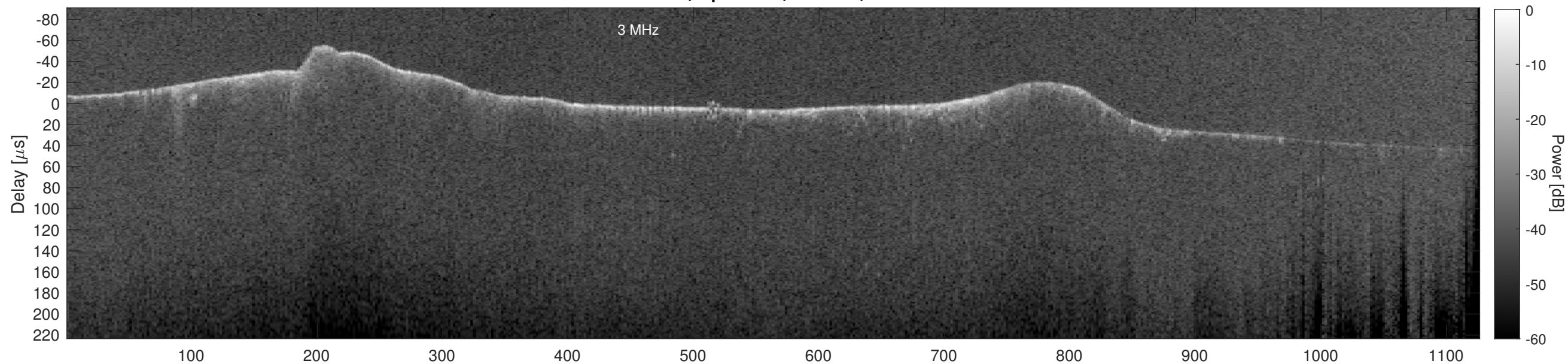
Orbit 12269, Cluttergram
