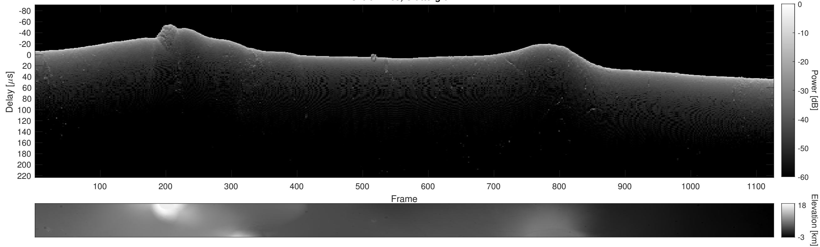
Orbit 12269, Cluttergram
