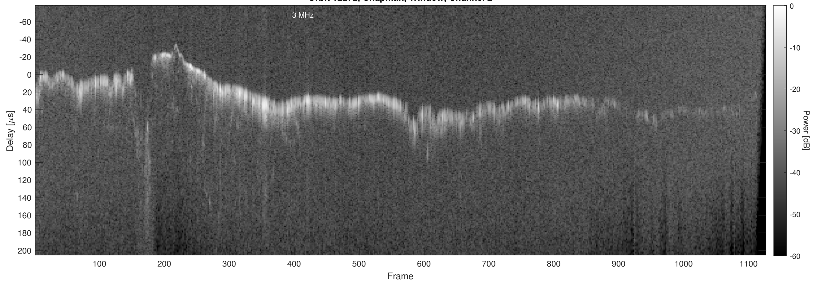
Orbit 12272, Chapman, Window, Channel 2
