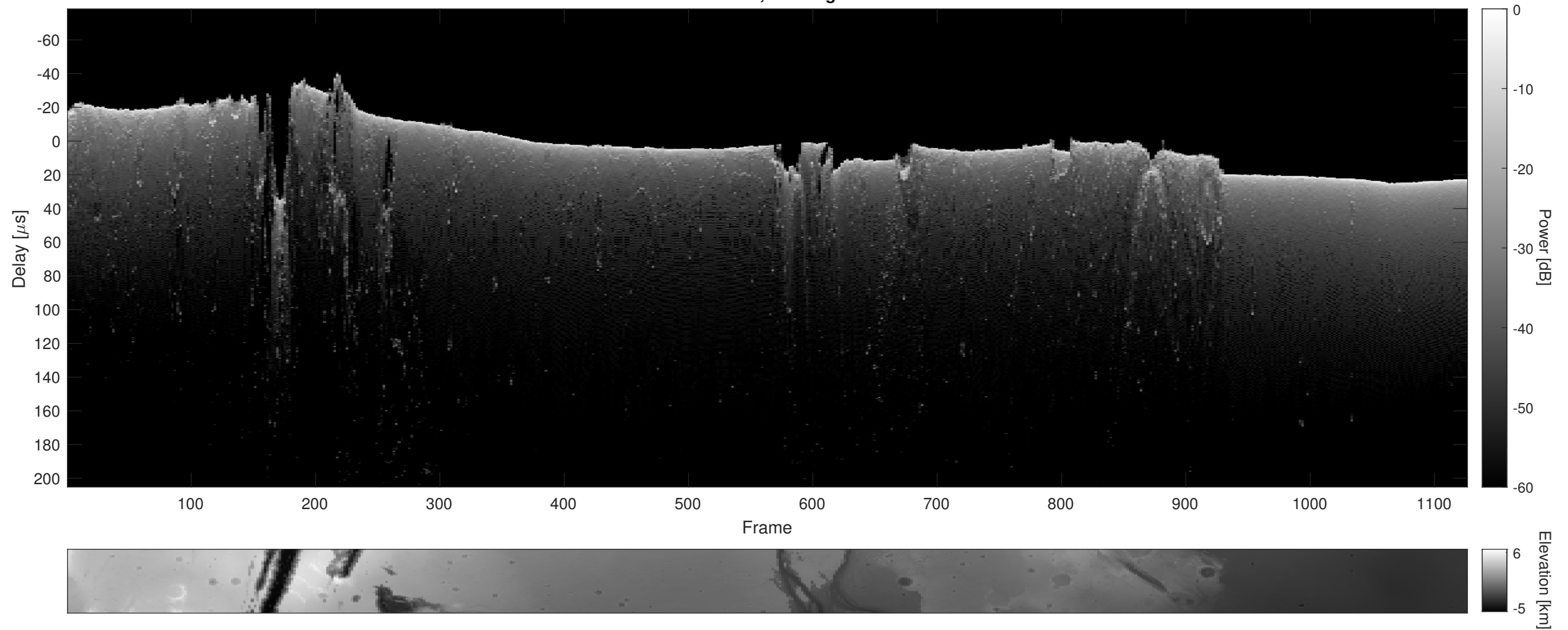
Orbit 12272, Cluttergram
