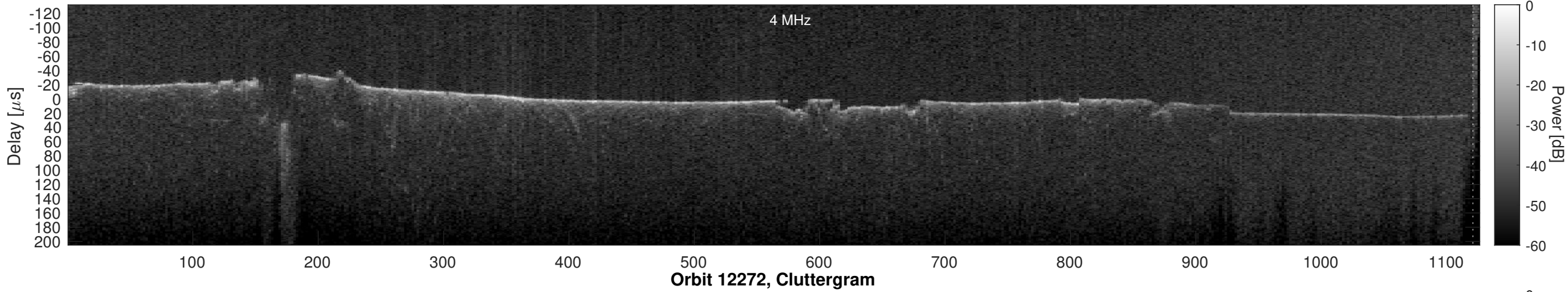
Orbit 12272, Window, Channel 1, Optimized
