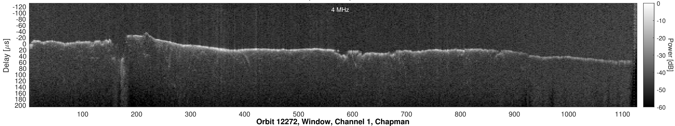
Orbit 12272, Channel 1, Uncorrected
