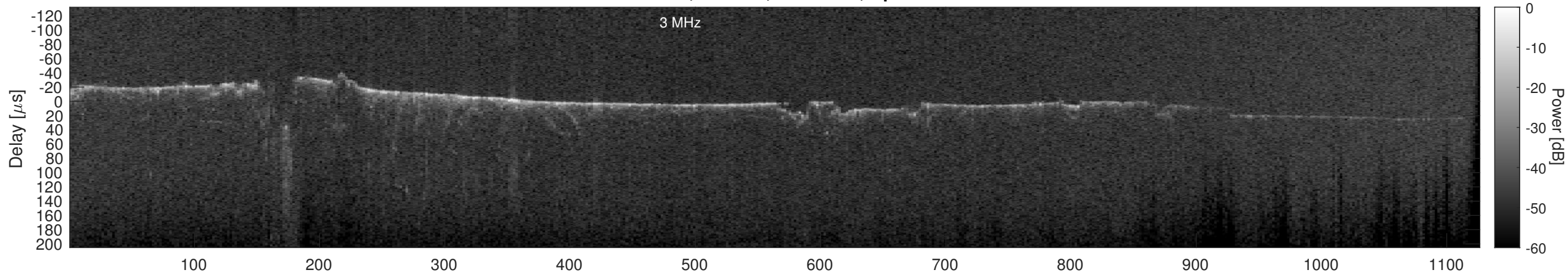
Orbit 12272, Cluttergram
