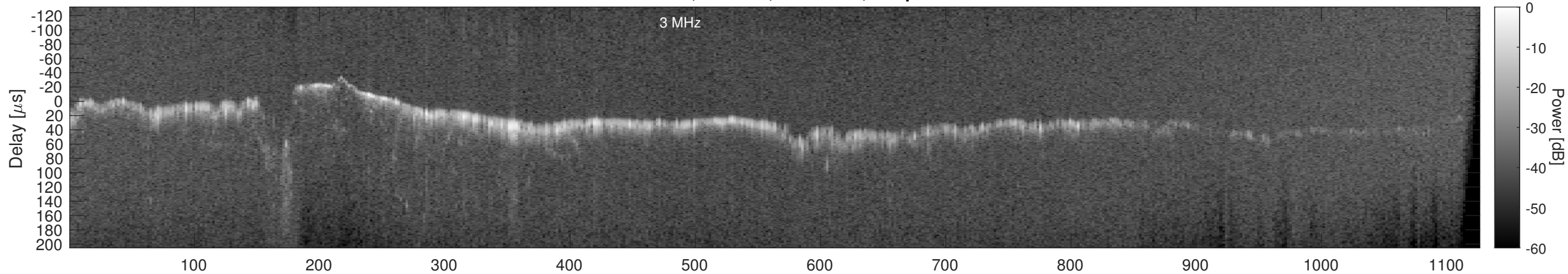
Orbit 12272, Window, Channel 2, Optimized
