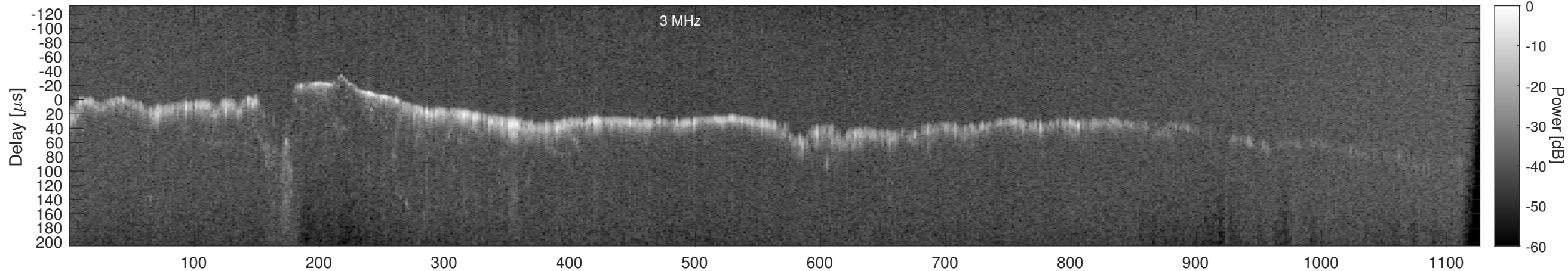
Orbit 12272, Window, Channel 2, Chapman
