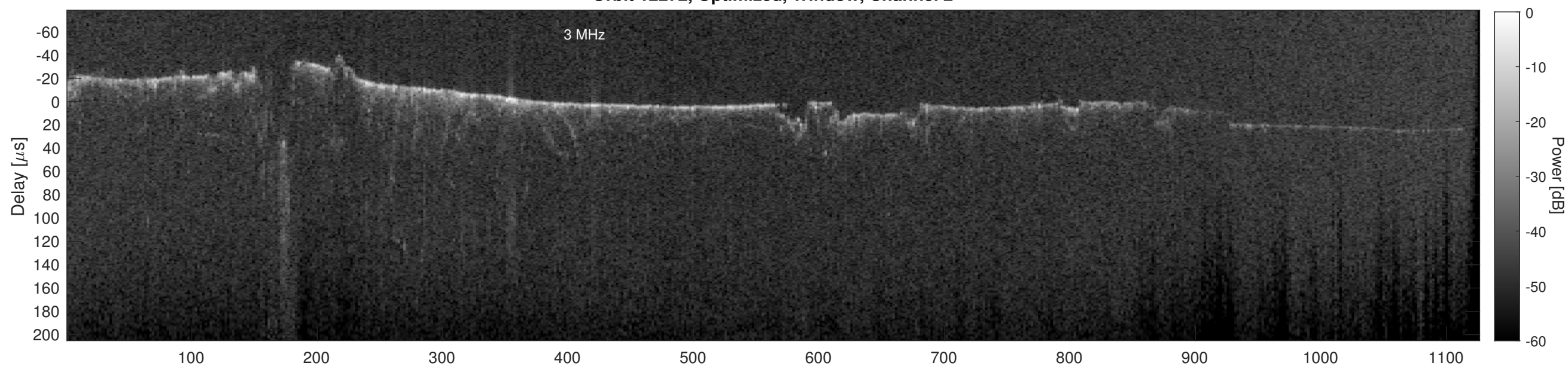
Orbit 12272, Cluttergram
