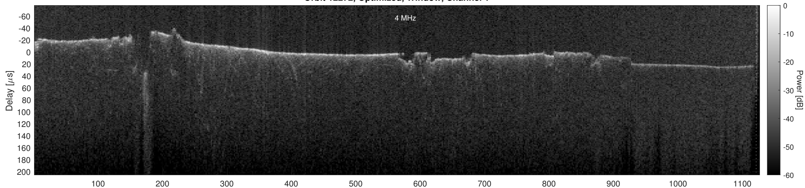
Orbit 12272, Optimized, Window, Channel 2
