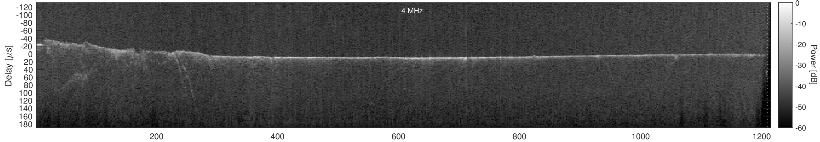
Orbit 12273, Cluttergram
