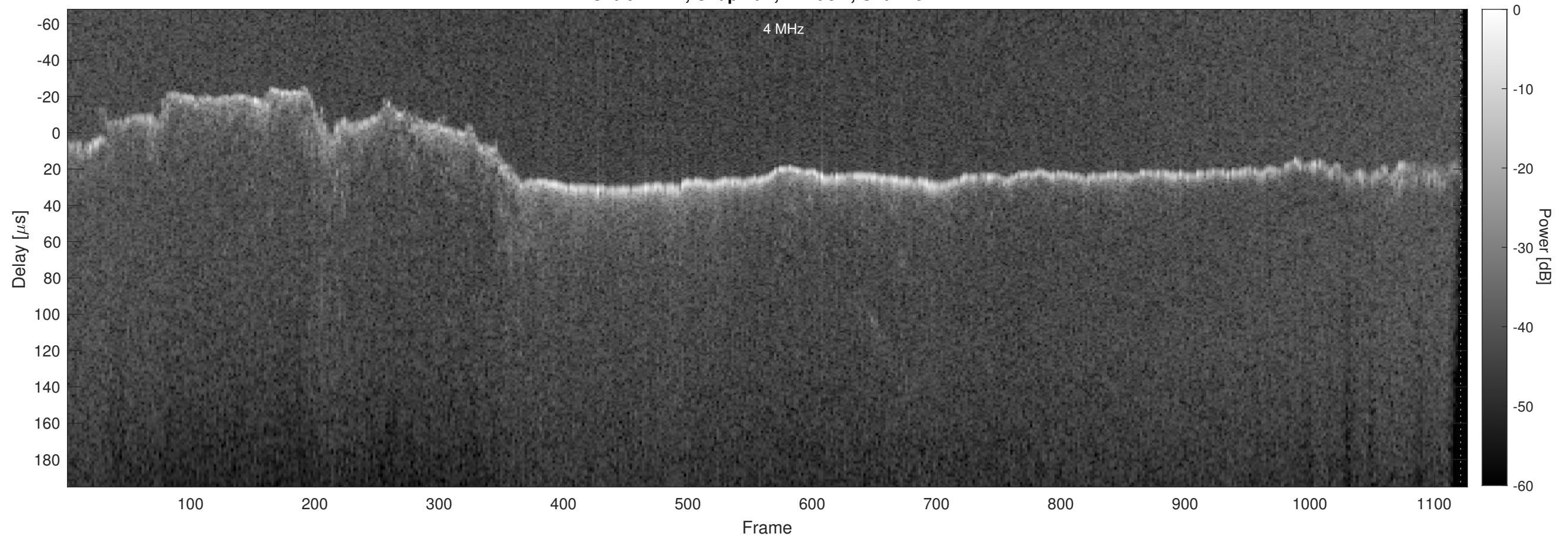
Orbit 12274, Chapman, Window, Channel 2
