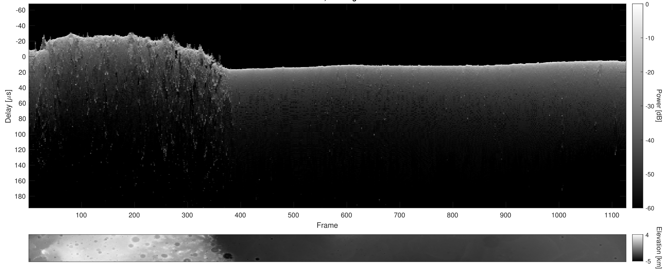
Orbit 12274, Cluttergram
