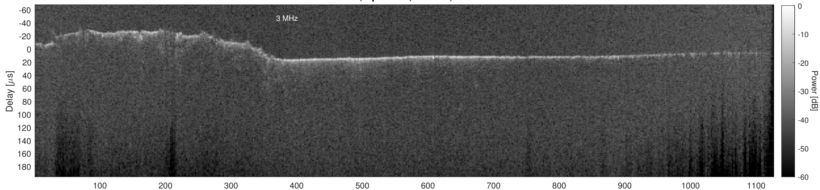
Orbit 12274, Cluttergram
