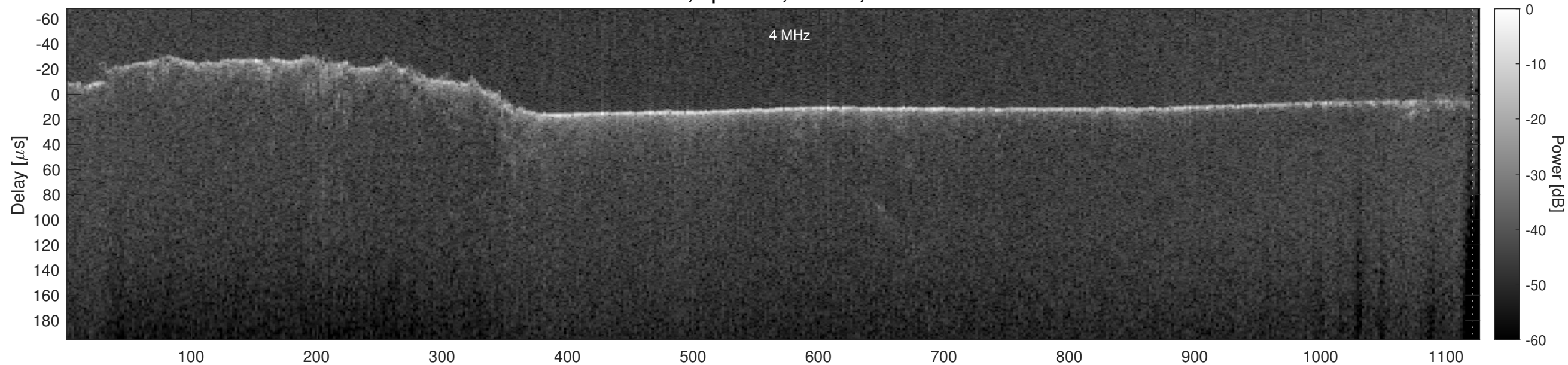
Orbit 12274, Optimized, Window, Channel 2
