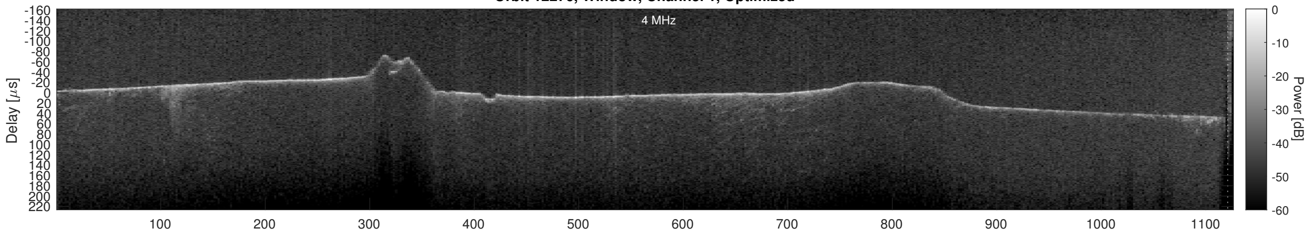
Orbit 12276, Cluttergram
