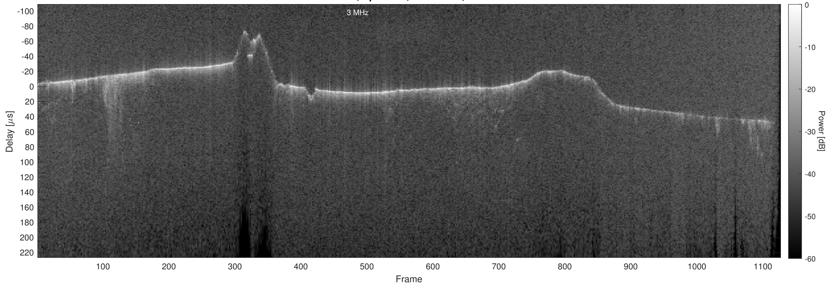
Orbit 12276, Optimized, No Window, Channel 2
