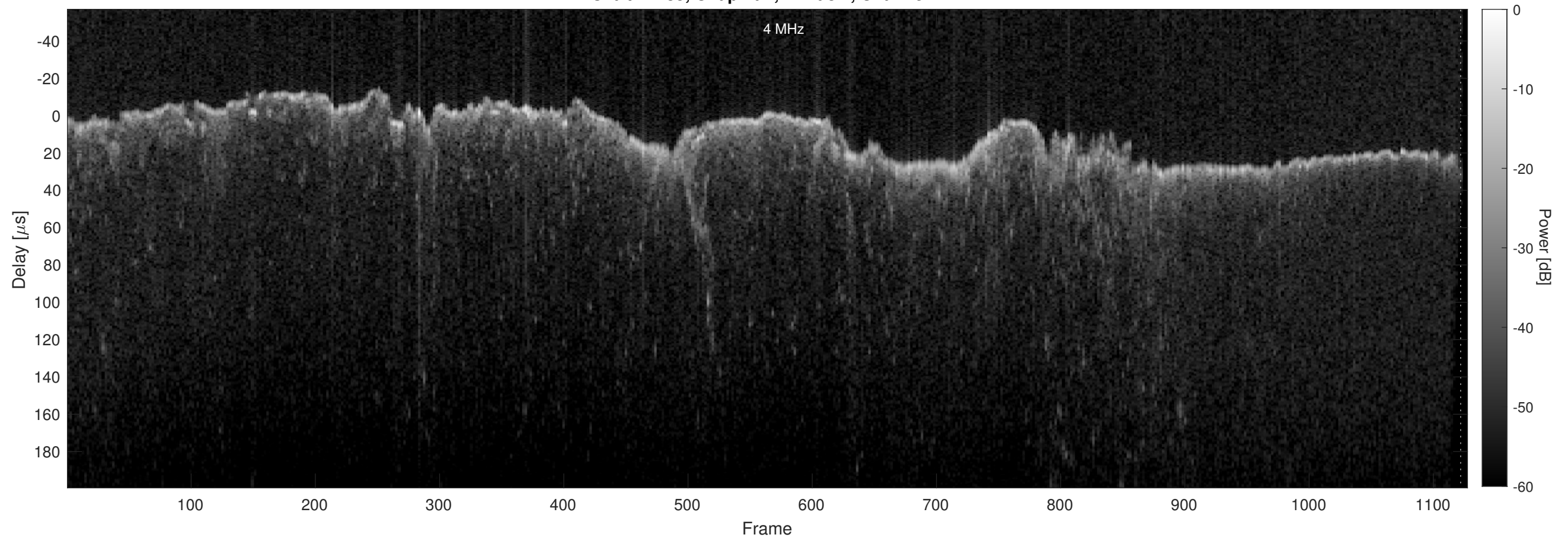
Orbit 12285, Chapman, Window, Channel 2
