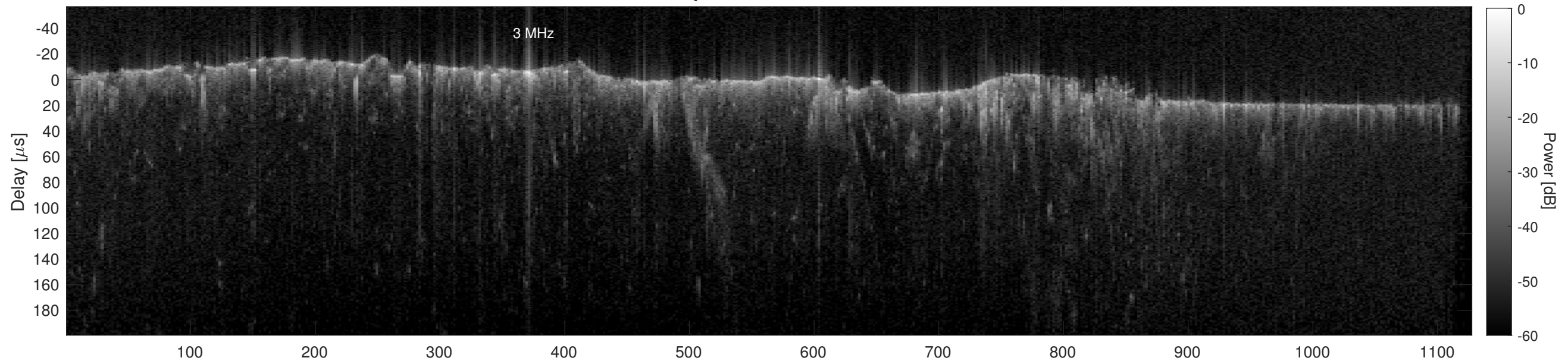
Orbit 12285, Cluttergram
